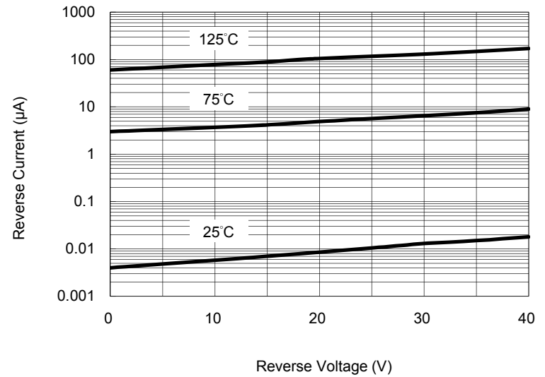
Fig. 2 Reverse Characteristics
