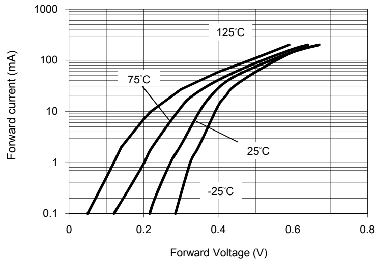
Fig.1 Forward Characteristics
