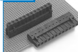
ELFB Inverted Header . . . . . Page 47 15A / 300V
