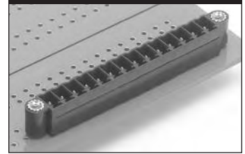
ELXH Vertical—Eared
