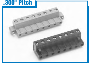
ELFP Right Angle . . . . . Page 50 ELFP with Locking Ears . . . Page 50 15A / 300V
