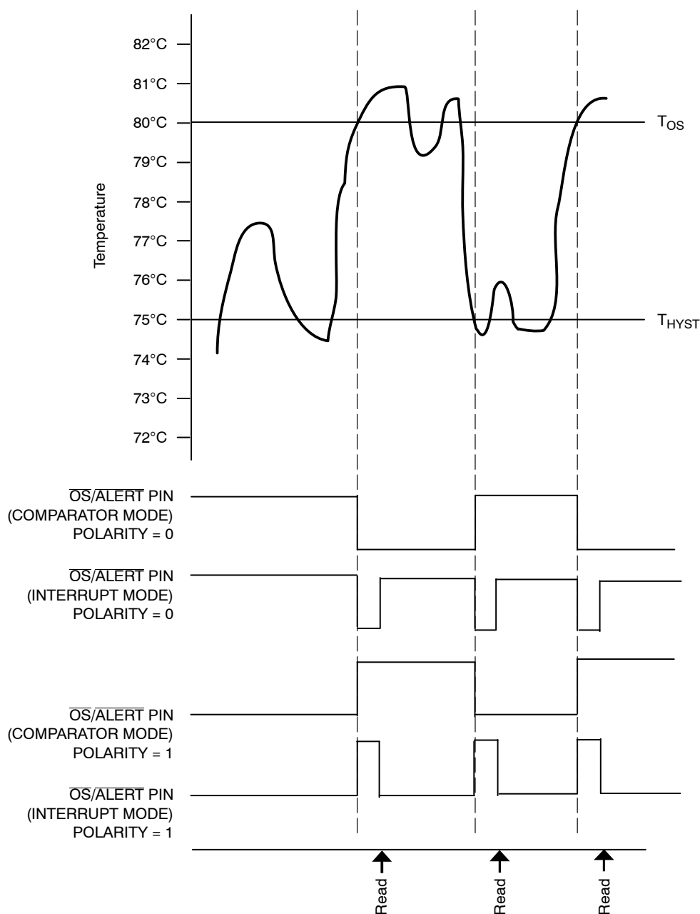
Figure 10. \overline{\text{OS/ALERT}} Output Temperature Response Diagram
