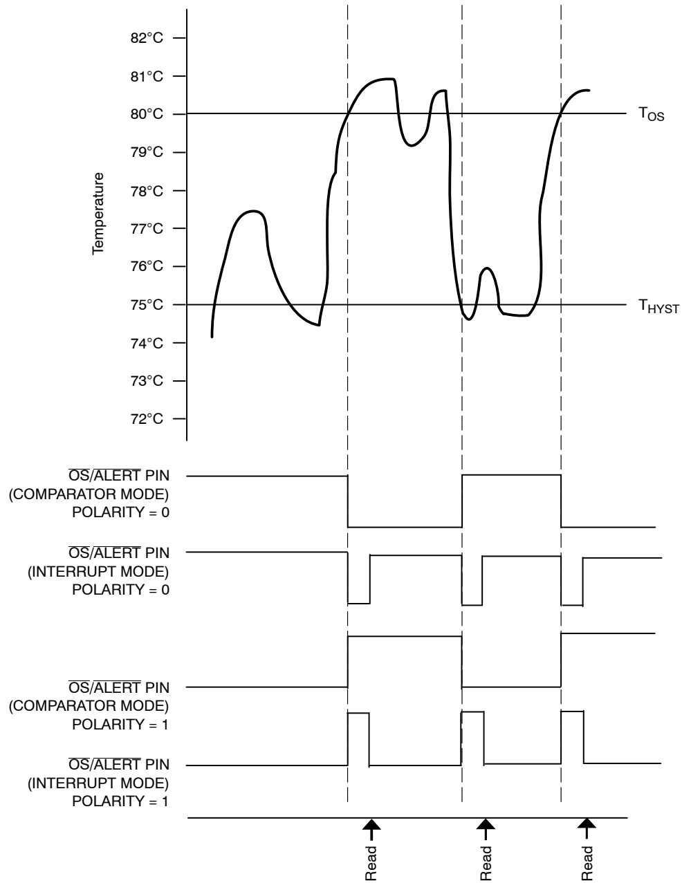
Figure 10. \overline{OS}/ALERT Output Temperature Response Diagram
