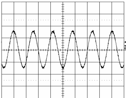
Output voltage ripple (20mV/div.) at: T_{ref} = +25^{\circ}\text{C} , I_O = 6\text{ A} resistive load, V_i = 12.0\text{ V} . Time scale: 2 μs/div. See the filter in the Output ripple and noise section (EMC Specification).
