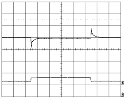
Output voltage response to load current step- Top trace: output voltage (100mV/div.). change (3-6-3 A) at: T_{ref} = +25^{\circ}\text{C} , V_i = 12.0\text{ V} . Bottom trace: load current (10 A/div.). Time scale: 0.1 ms/div.
