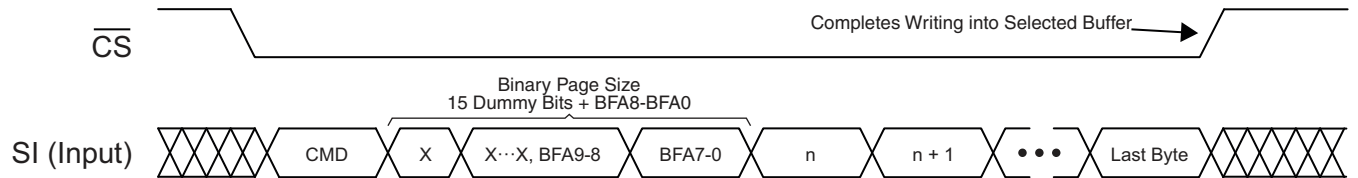
Figure 22-2. Buffer Write
