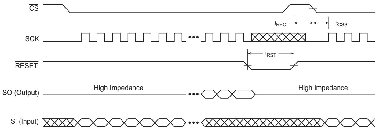
Figure 24-12. Reset Timing
