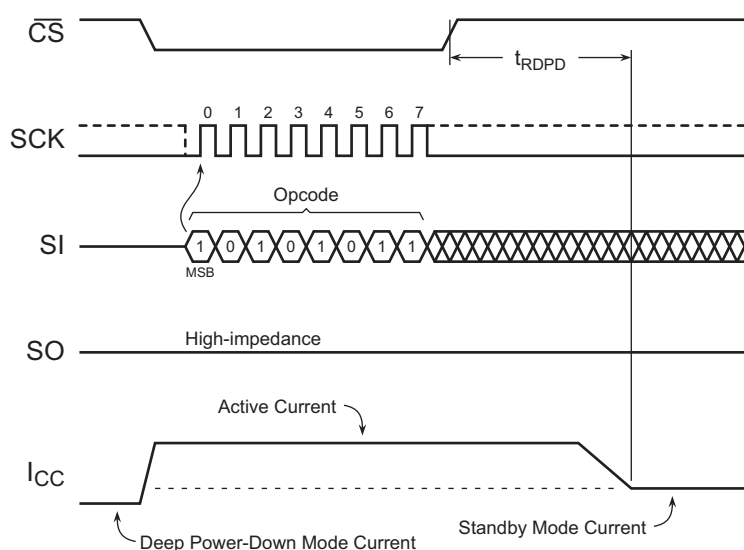
Figure 9-2. Resume from Deep Power-Down
