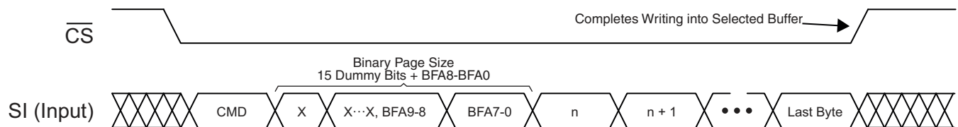
Figure 22-2. Buffer Write
