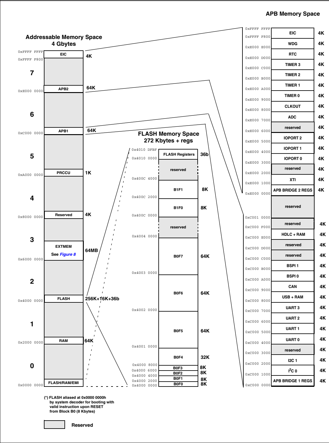
Figure 6. Memory map
