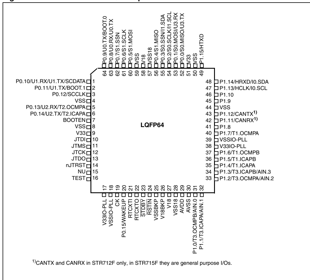
Figure 3. STR712/STR715 LQFP64 pinout
