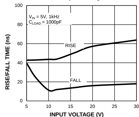
Rise/Fall Time vs. Input Voltage
