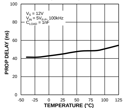
Enable-to-Output Propagation Delay vs. Temperature
