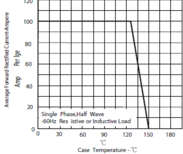
Figure.2-Forward Derating Curve
