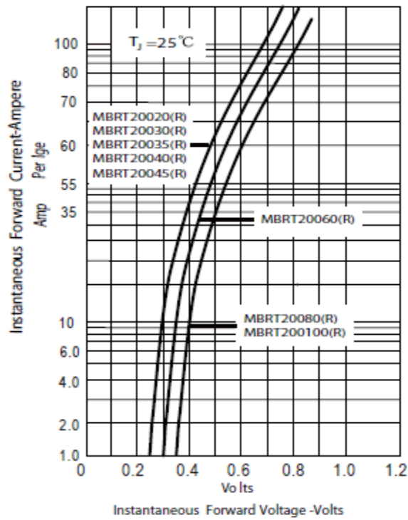
Figure.1-Typical Forward Characteristics
