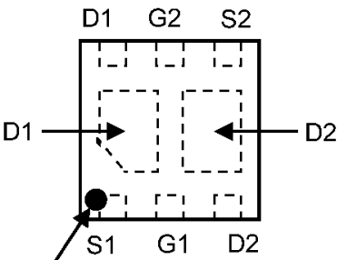
Fig. 6.1 Marking
