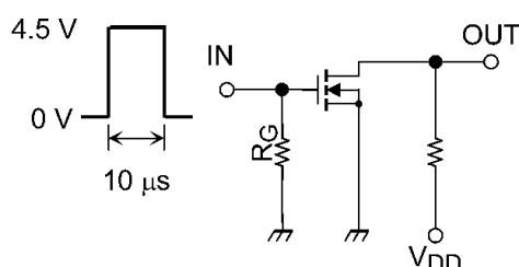
Fig. 5.3.1 Test Circuit of Switching Time
