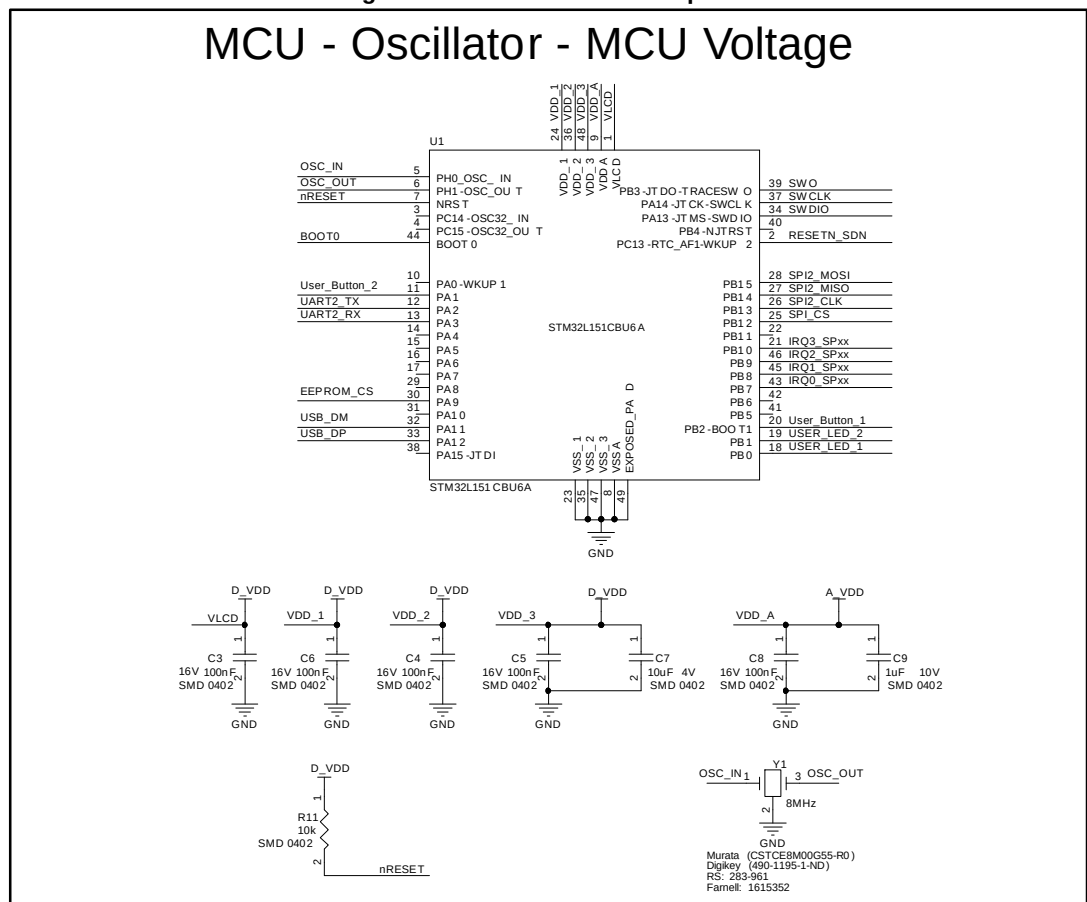
Figure 3: STEVAL-IDS001V4M part 3
