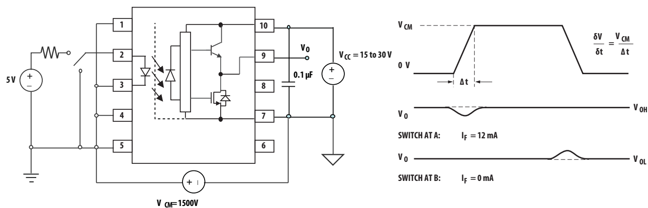
Figure 23. CMR test circuit and waveforms
