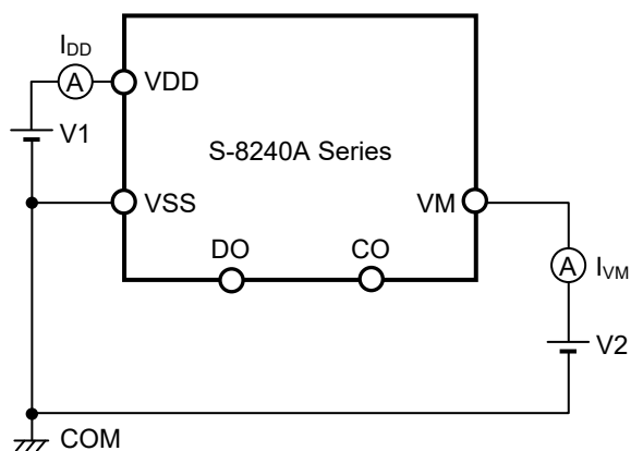
Figure 8 Test Circuit 3
