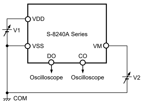
Figure 10 Test Circuit 5
