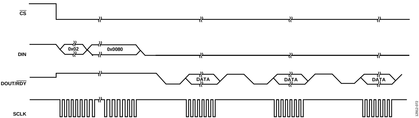
Figure 67. Continuous Read Mode
