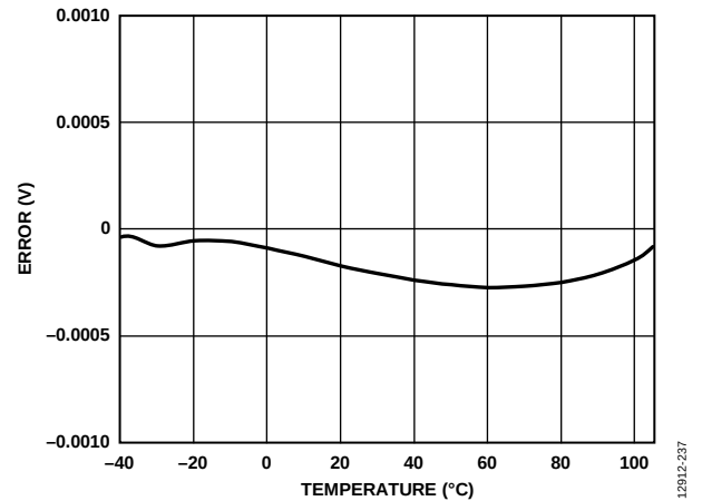
Figure 27. Absolute Reference Error vs. Temperature
