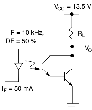
Fig. 9 - Switching Schematic
