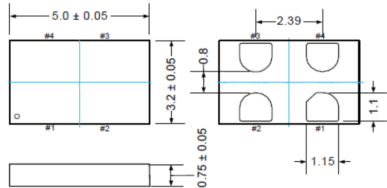
5.0 x 3.2mm Package (Option “FL”)
