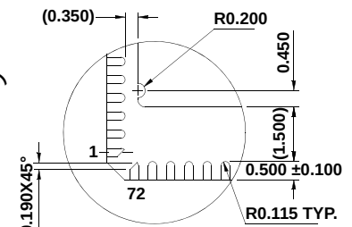
DETAIL "Z"
