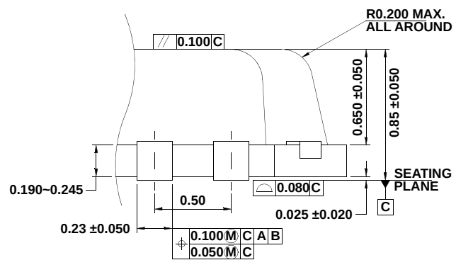
DETAIL "Y"
