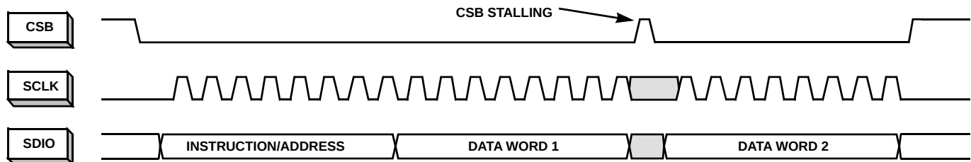
FIGURE 39. SPI READ
