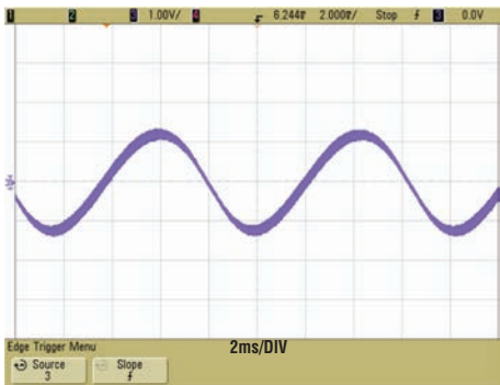
Figure 11. Output Ripple at 120VAC, 2A Load
