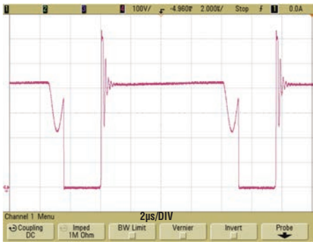
Figure 8. 230VAC ( V_{SW} = 630V )
