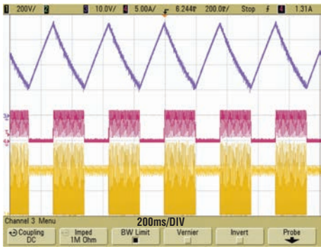
Figure 10. 230VAC
