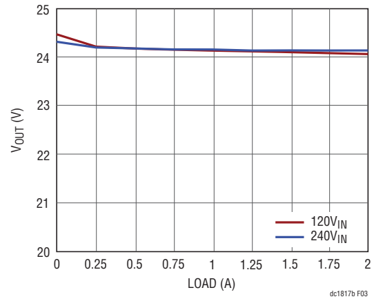
Figure 3. V OUT vs Load Current
