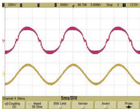
Figure 5. 120VAC (PF = 0.99)
