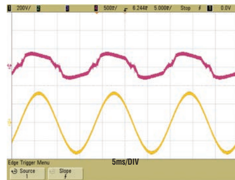
Figure 6. 230VAC (PF = 0.97)
