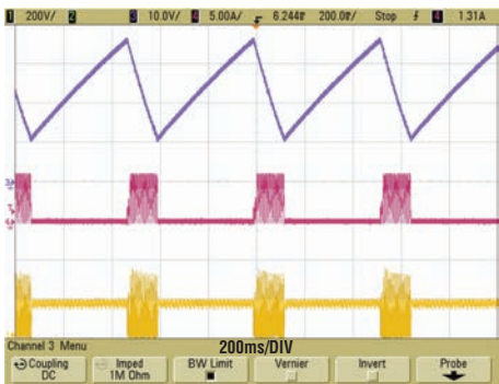
Figure 9. 120VAC
