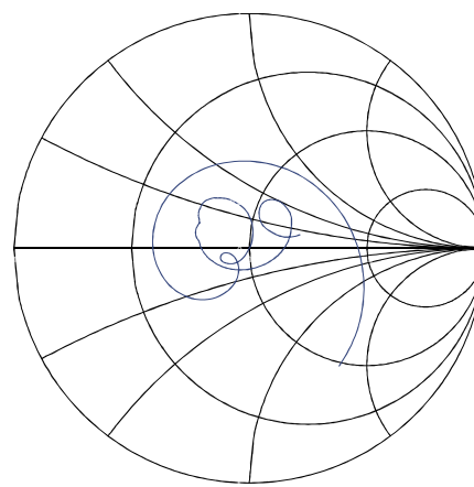
Output Smith Chart
