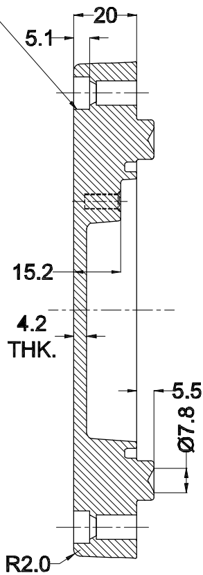
SECTION B-B
