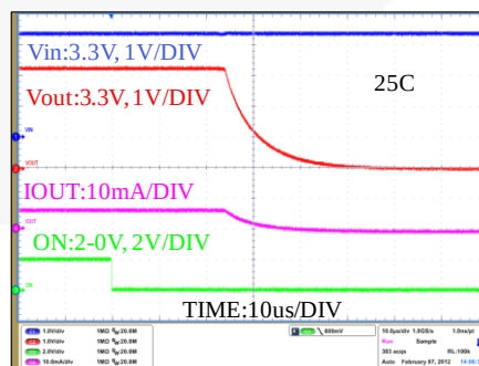
Figure 23. Turn-Off Response ( V_{IN}=3.3\ \text{V} , C_{OUT}=0.1\ \mu\text{F} , R_L=500\ \Omega )
