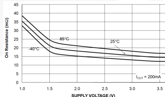
Figure 15. R_{ON} vs. Supply Voltage
