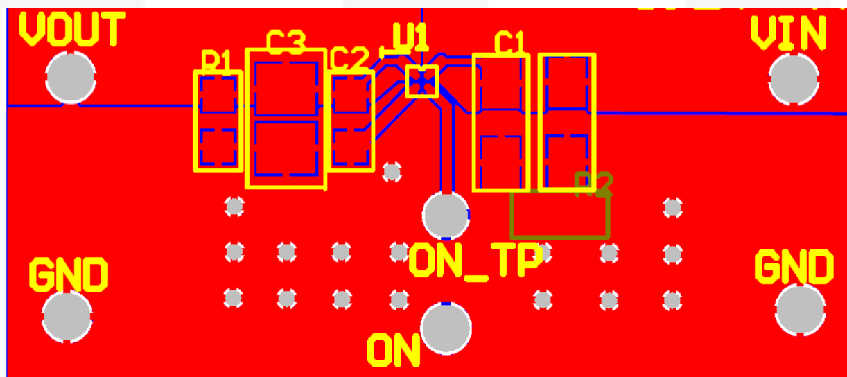
Figure 24. Recommended Land Pattern and Layout
