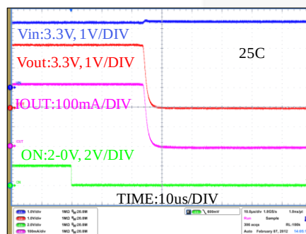
Figure 21. Turn-Off Response ( V_{IN}=3.3\ \text{V} , C_{OUT}=0.1\ \mu\text{F} , R_L=10\ \Omega )
