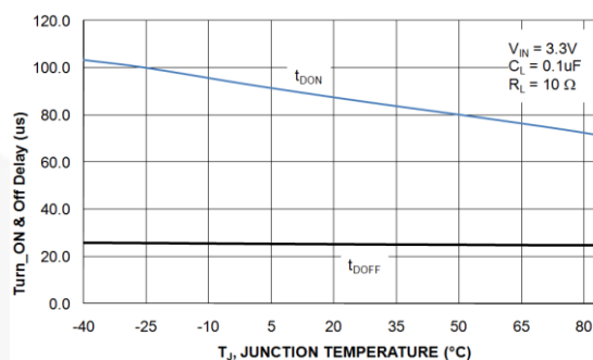
Figure 17. V_{OUT} Turn-On/Turn-Off Delays vs. Temperature ( R_L=10\ \Omega )
