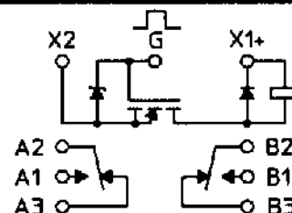
TERMINAL VIEW
