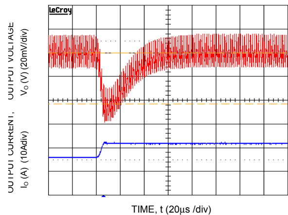
Figure 22. Transient Response to Dynamic Load Change from 50% to 100% at 12Vin, C_{out}=1x47\mu F+1x330\mu F , C_{Tune}=3300pF & R_{Tune}=270ohms
