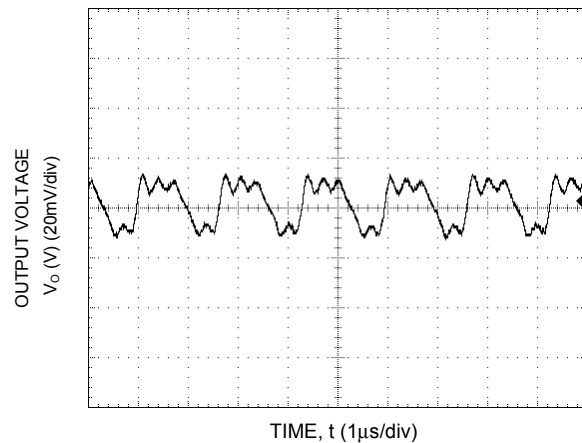
Figure 15. Typical output ripple and noise ( C_o=22\mu F ceramic, V_{in} = 12V , I_o = I_{o,max} ).
