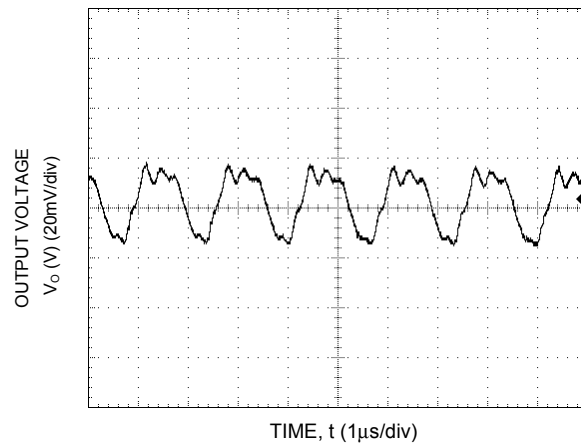
Figure 21. Typical output ripple and noise ( C_O=22\mu F ceramic, V_{IN} = 12V , I_o = I_{o,max} ).
