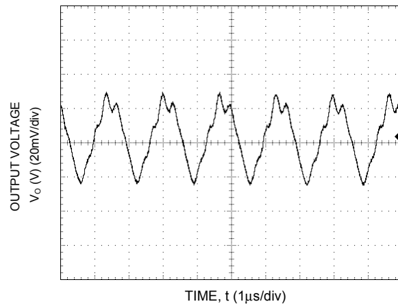
Figure 33. Typical output ripple and noise (C o =22μF ceramic, V IN = 12V, I o = I o,max ).
