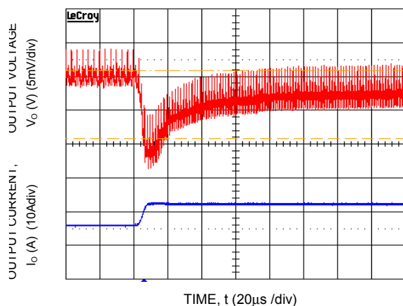
Figure 4. Transient Response to Dynamic Load Change from 50% to 100% at 12Vin, C out =3x47μF+6x330μF, C Tune =47nF, R Tune =180ohms
