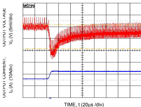
Figure 4. Transient Response to Dynamic Load Change from 50% to 100% at 12Vin, Cout=3x47uF+6x330uF, CTune=47nF, RTune=180ohms
