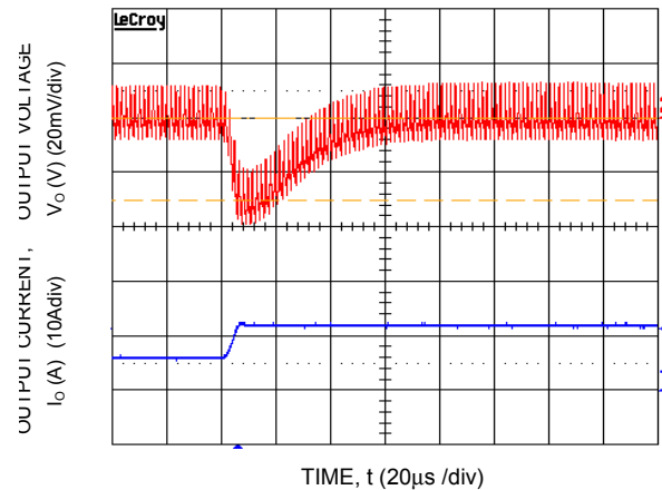
Figure 16. Transient Response to Dynamic Load Change from 50% to 100% at 12Vin, C_{out}=1x47\mu F+2x330\mu F , C_{Tune}=5600pF & R_{Tune}=270ohms
