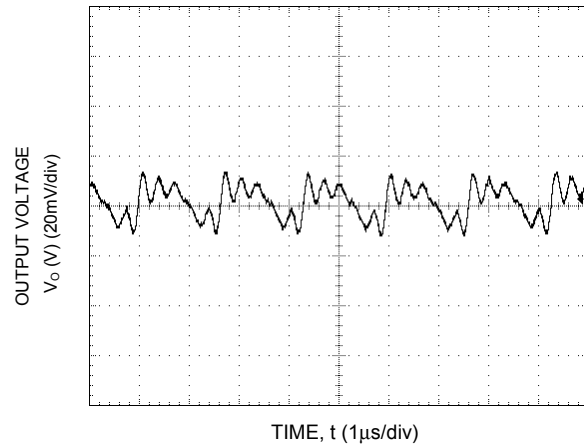
Figure 9. Typical output ripple and noise ( C_O=22\mu F ceramic, V_{IN} = 12V , I_o = I_{o,max} ).
