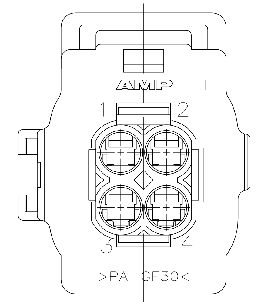
VIEW B-B
