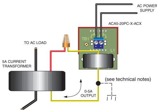
Figure 1. Typical Connections
