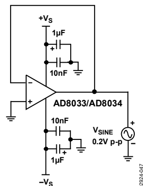
Figure 47. Output Impedance, G = +1
