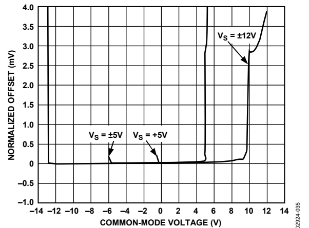
Figure 35. Input Offset Voltage vs. Common-Mode Voltage
