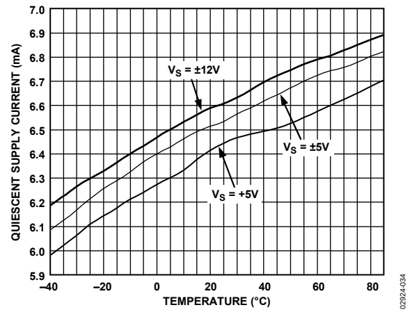
Figure 34. Quiescent Supply Current vs. Temperature for Various Supply Voltages
