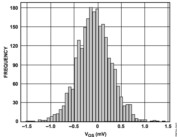
Figure 41. Initial Offset
