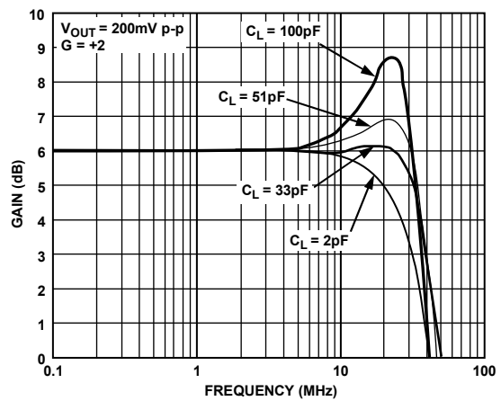
Figure 15. Small Signal Frequency Response for Various C_L (See Figure 45)
