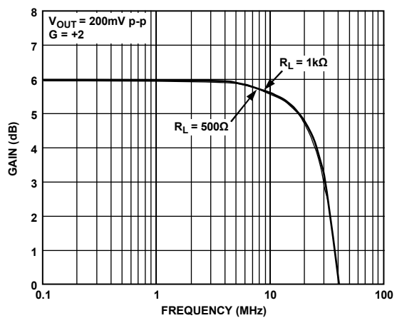
Figure 16. Small Signal Frequency Response for Various R_L (See Figure 45)
