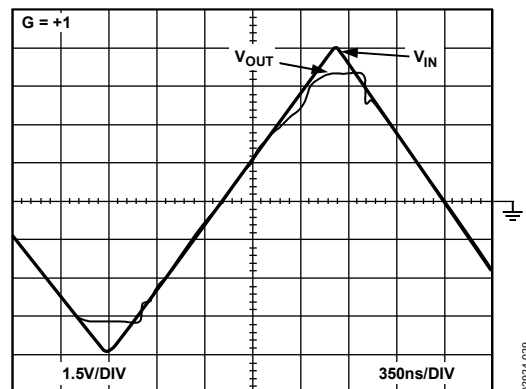
Figure 29. Input Overdrive Recovery (See Figure 44)
