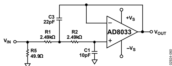
Figure 60. 2-Pole Butterworth Active Filter
