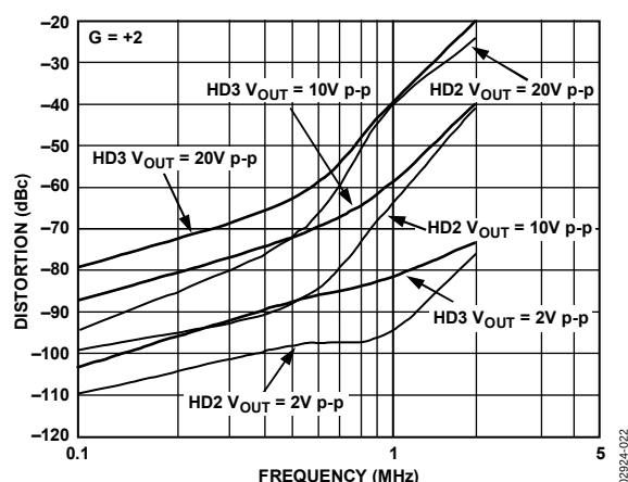
Figure 22. Harmonic Distortion vs. Frequency for Various Amplitudes (See Figure 45), V_S = 24\text{ V}
