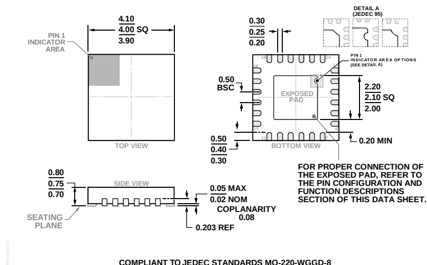
Figure 45. 24-Lead Lead Frame Chip Scale Package [LFCSP] 4 mm × 4 mm Body and 0.75 mm Package Height (CP-24-10) Dimensions shown in millimeters
