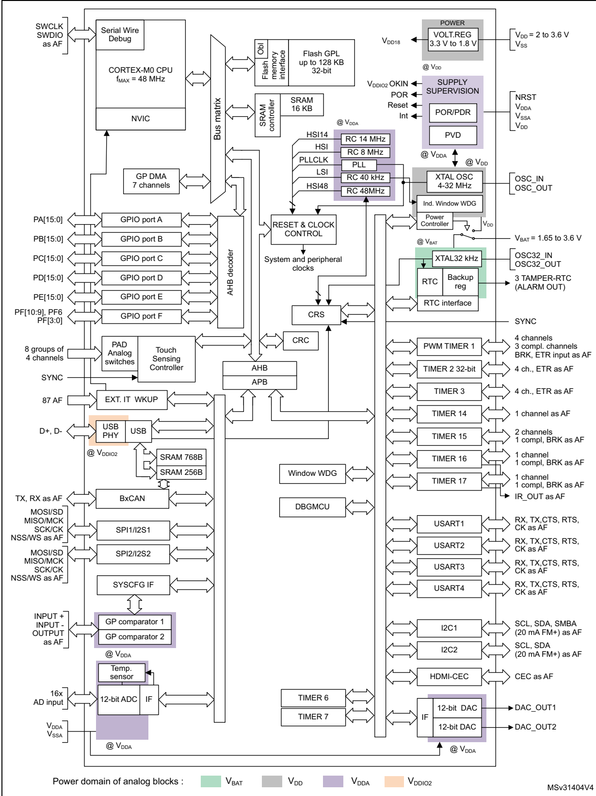
Figure 1. Block diagram
