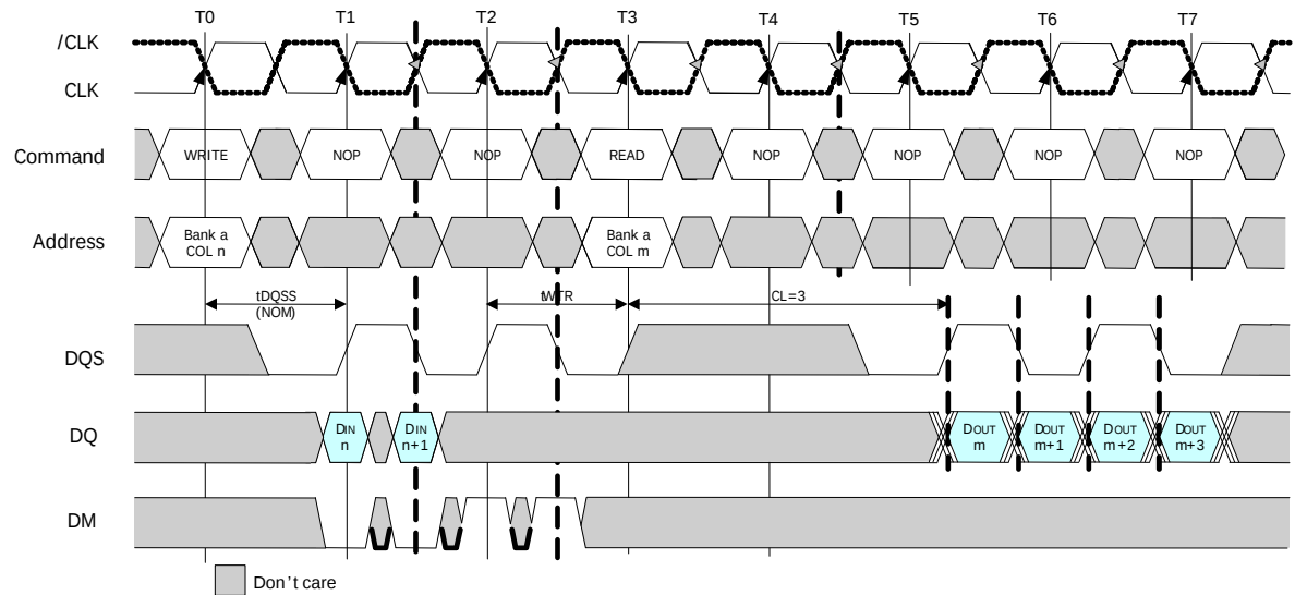
Figure27 : Write to Read (Interrupting)
