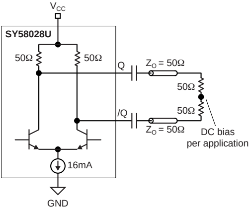
Figure 5b. CML AC-Coupled (50Ω Termination)
