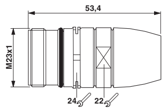
Dimensional drawing
