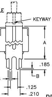
FRONT VIEW DOUBLE POLE
