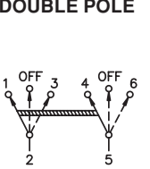
DOUBLE POLE
