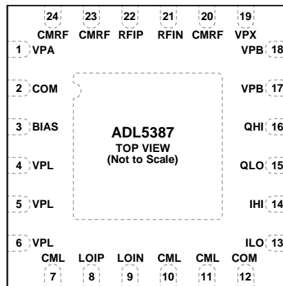
Figure 2. Pin Configuration
