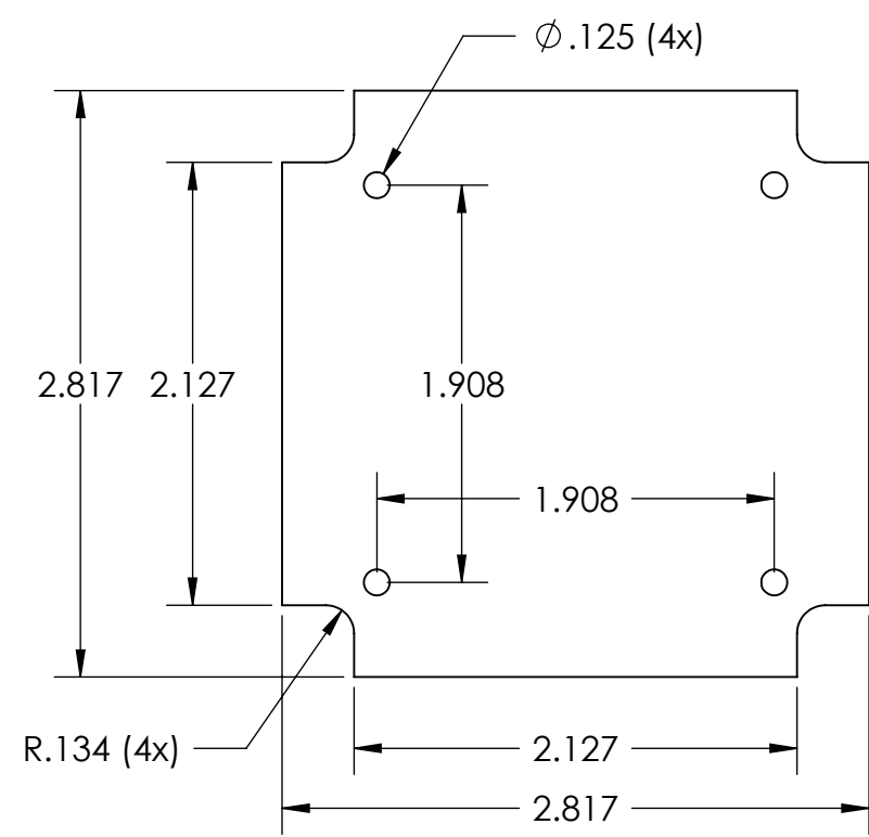
SUGGESTED PC BOARD LAYOUT
