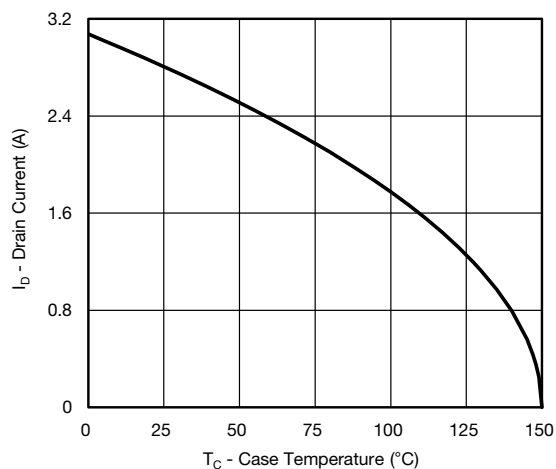
Max Current vs. Case Temperature
