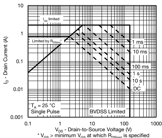
Safe Operating Area at T_A = 25\text{ }^{\circ}\text{C}
