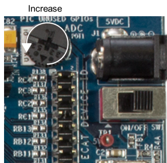
FIGURE 2-8: POTENTIOMETER POT1
