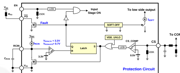
Figure 42. Over-Current Protection
