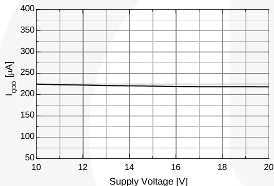
Figure 30. Quiescent V_{DD} Supply Current vs. Supply Voltage
