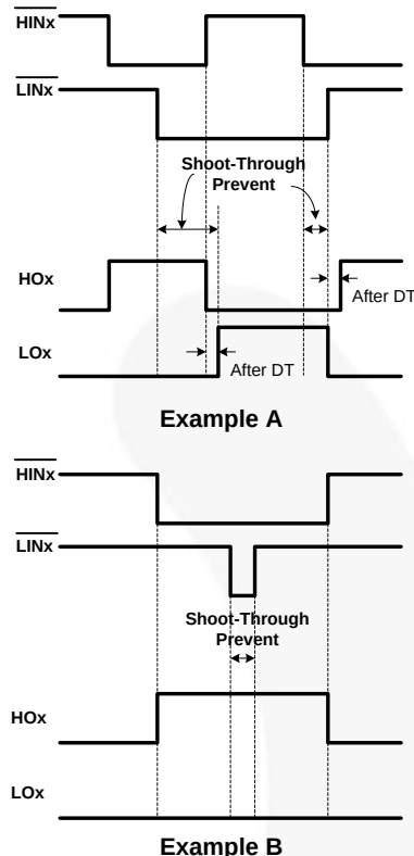
Figure 39. Shoot-Through Protection
