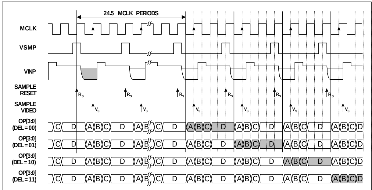
Figure 15 Mode 2 Operation
