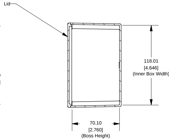
SECTION A-A End View of Assembly
