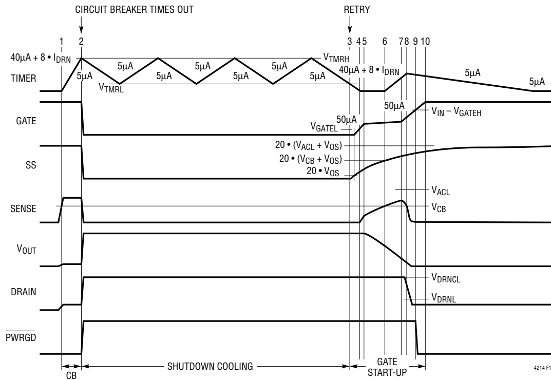
Figure 15. Shutdown Cooling Timing Behavior of LTC4214-2 (All Waveforms are Referenced to V_{EE} )
