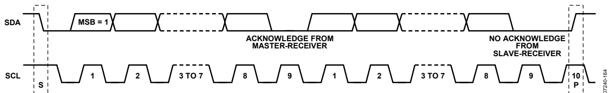
Figure 47. Data Transfer Process (Master Read Mode, 2-Byte Transfer Used for Illustration)
