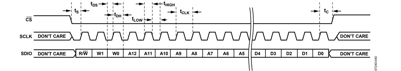
Figure 53. Serial Control Port Write—MSB First, 16-Bit Instruction, Timing Measurements
